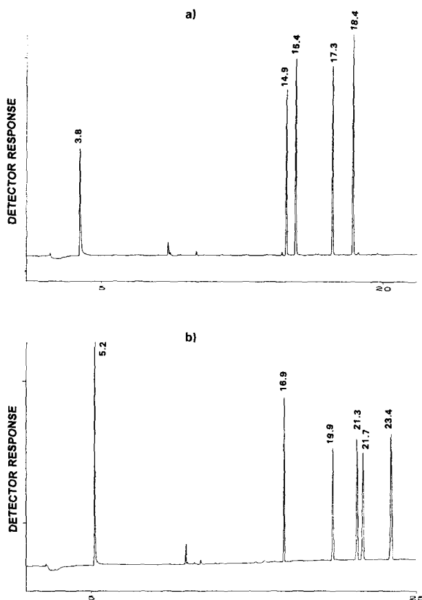
Figure 2. Chromatograms for the separation of six OPs. a) in Ultra 2® column, in order of elution: Trichlorfon, 10 ng; Phorate, 10 ng; Dimethoate, 10 ng; Parathion-methyl, 10 ng; Parathion, 10 ng (Chlorpyrifos elutes at the same retention time). b) in SGE-1701® column, in order of elution: Trichlorfon, 50 ng; Phorate, 5 ng; Dimethoate, 10 ng; Chlorpyrifos 10 ng; Parathion-Methyl, 20 ng; Parathion, 10 ng.
