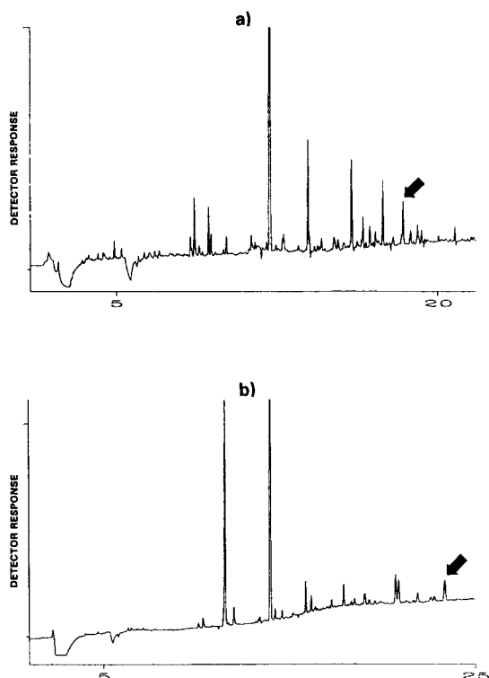
Figure 3. Chromatograms of an extract of environmental water taken in November 1990 from station 2, which contained 0.204 \mu\text{g/L} Parathion. a) in Ultra 2® column. b) in SGE-1701® column. Parathion is indicated with the arrows.
